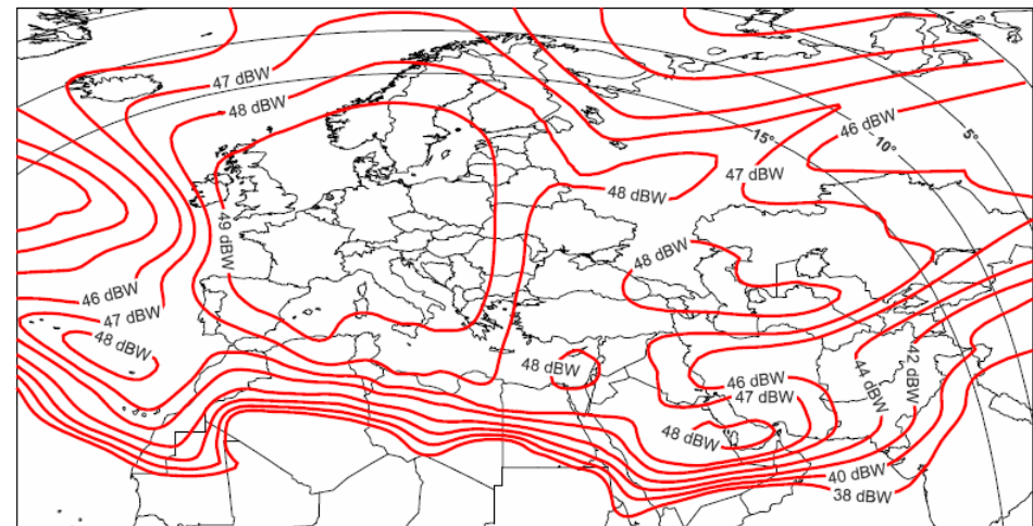
Figure 2 : Eutelsat 16A Illustration of Europe-A Transmit Coverage (not contractual)
